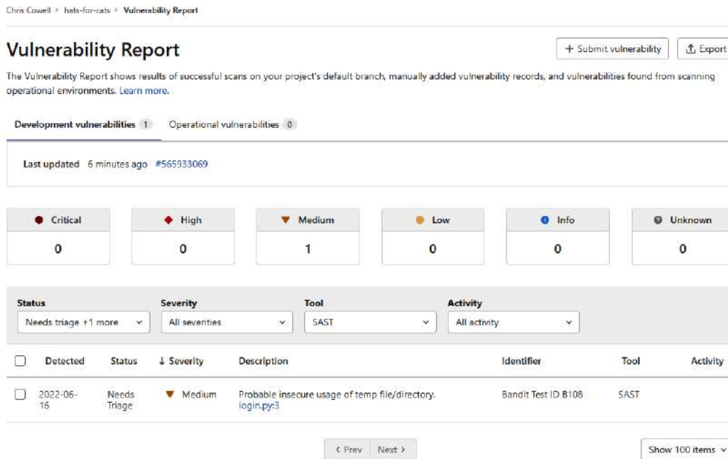
Figure 7.2 – SAST finding
