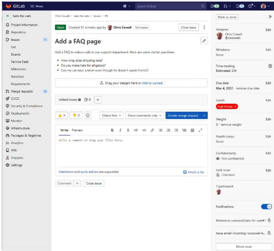
Figure 3.4 – Sample issue
