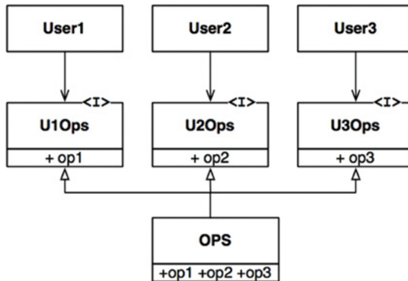
Figure 10.2 Segregated operations
