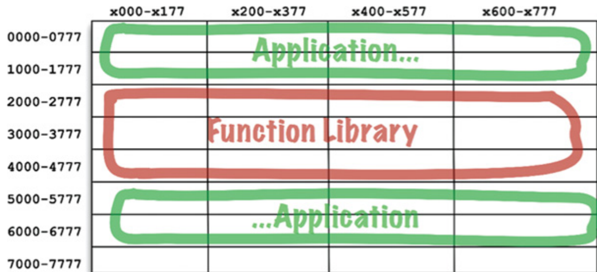
Figure 12.2 Splitting the application into two address segments
