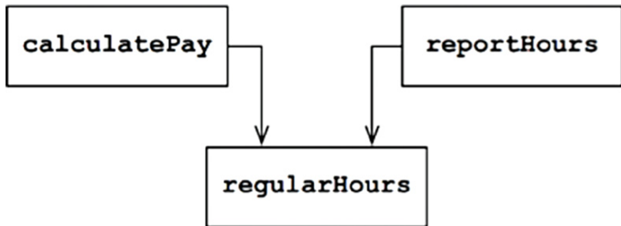
Figure 7.2 Shared algorithm
