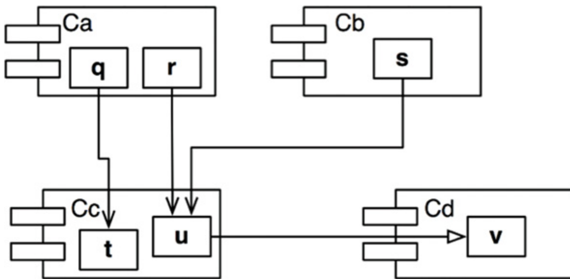
Figure 14.7 Our example
