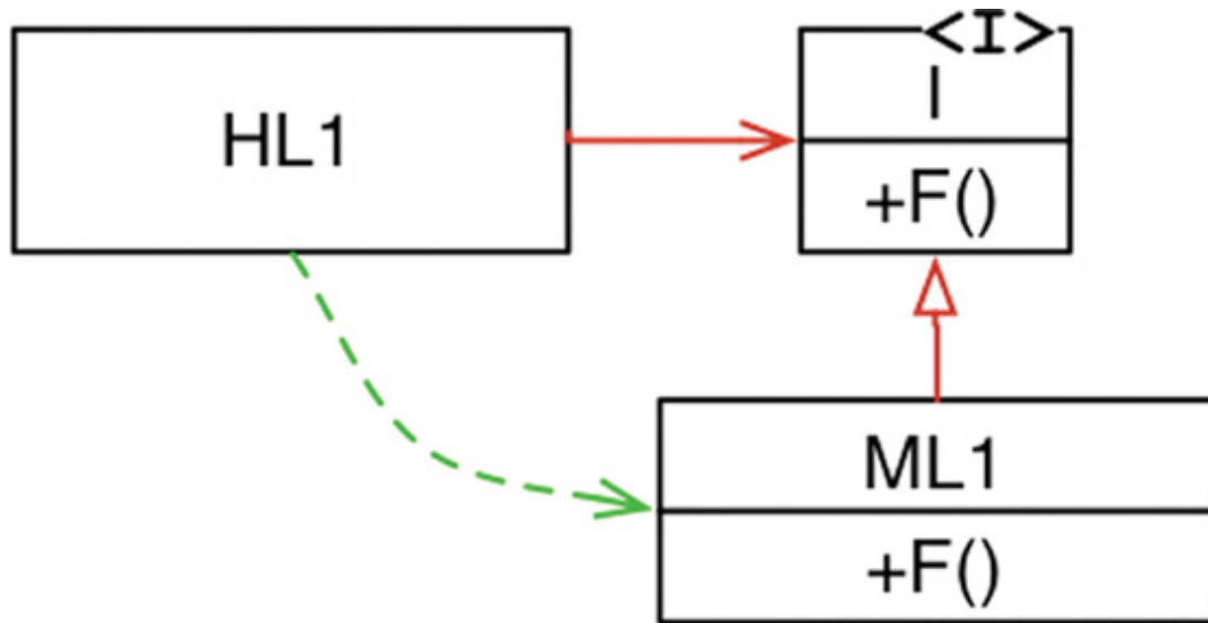
Figure 5.2 Dependency inversion
