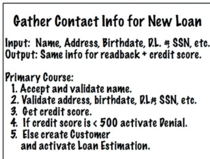
Figure 20.2 Example use case
