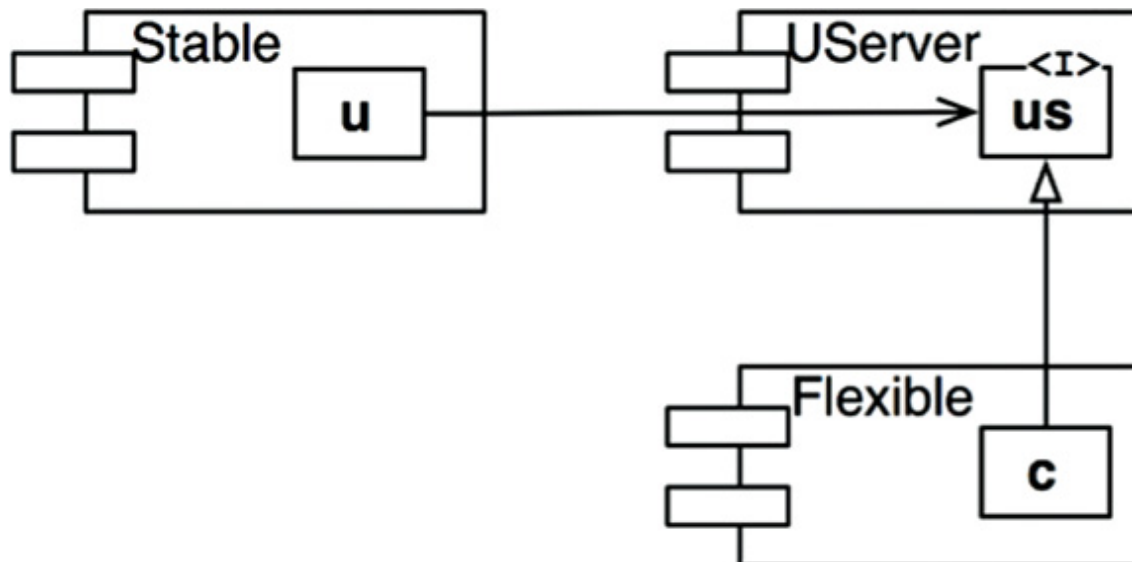
Figure 14.11 C implements the interface class US
