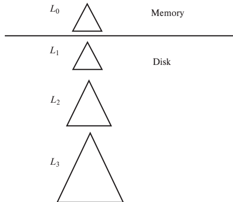
Figure 24.1 Log-structured merge tree with three levels.
