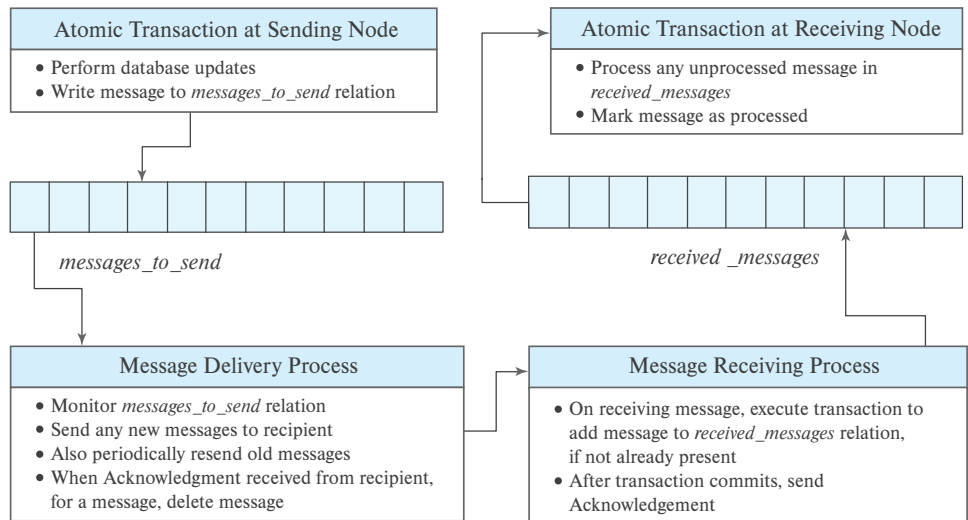
Figure 23.3 Implementation of persistent messaging.
