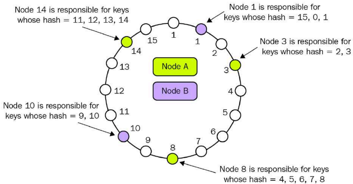
Figure 7.3 – Cassandra replication
