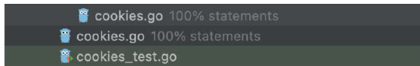
Figure 8.5 – 100% test coverage!
