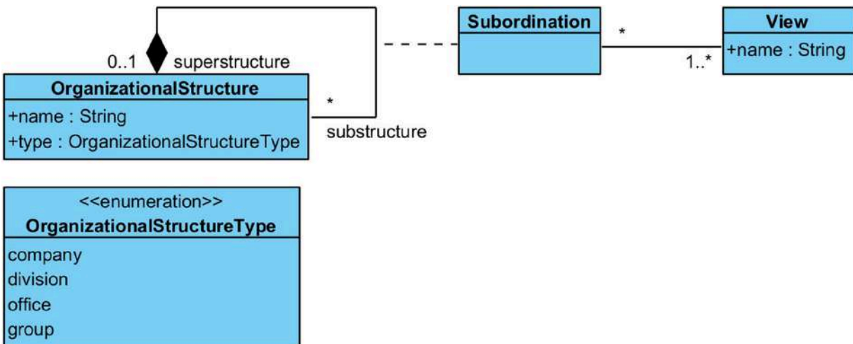
FIGURE 11-24 Parallel hierarchies.
