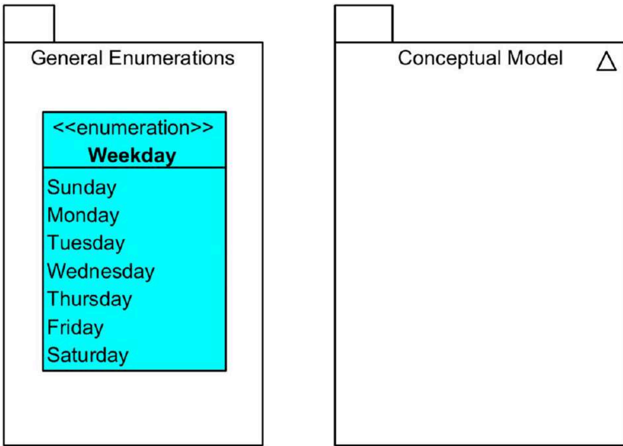
FIGURE 8-5 Enumeration.
