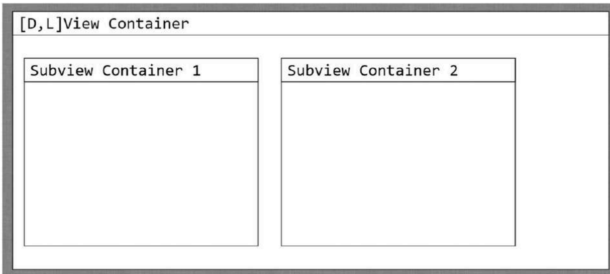
FIGURE 16–1 View containers.
