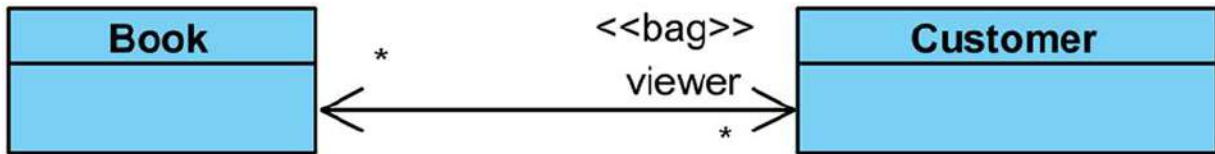
FIGURE 17–6 A bag.
