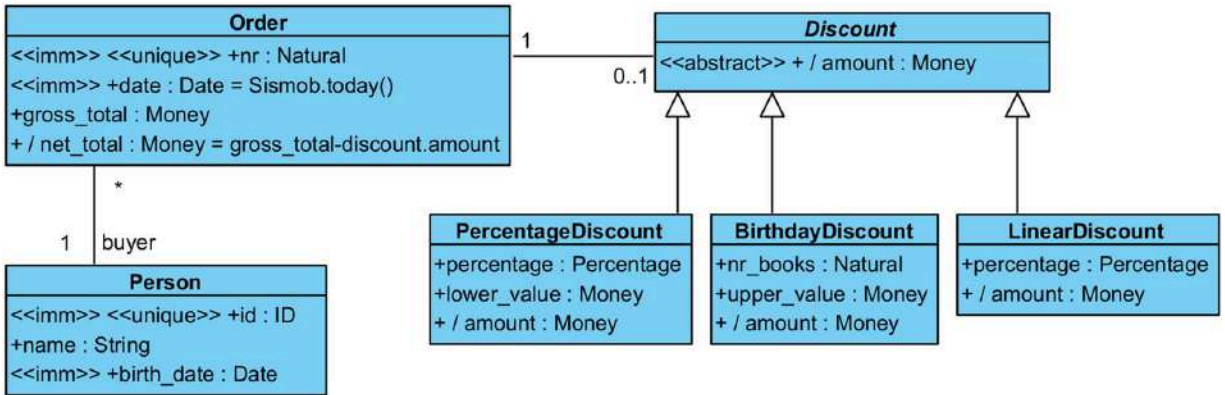
FIGURE 11–19 Strategy pattern.
