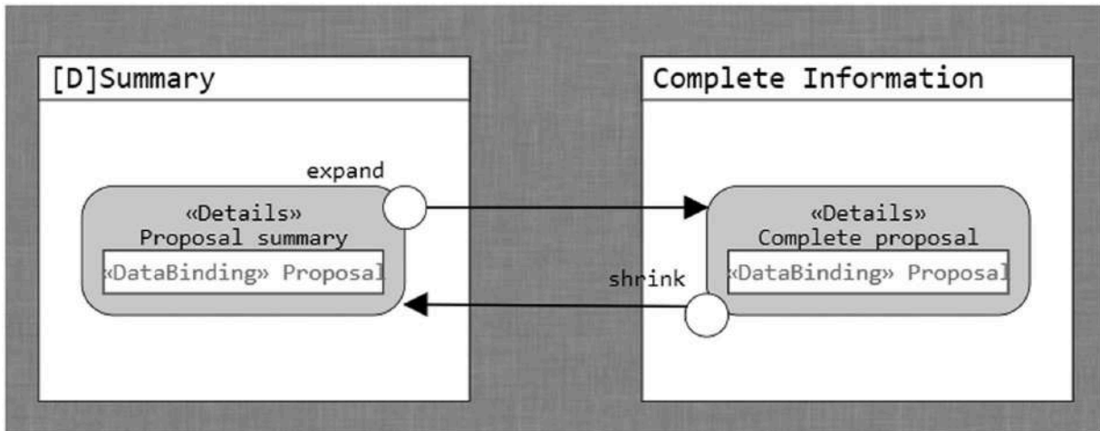
FIGURE 16-18 Viewpoints.
