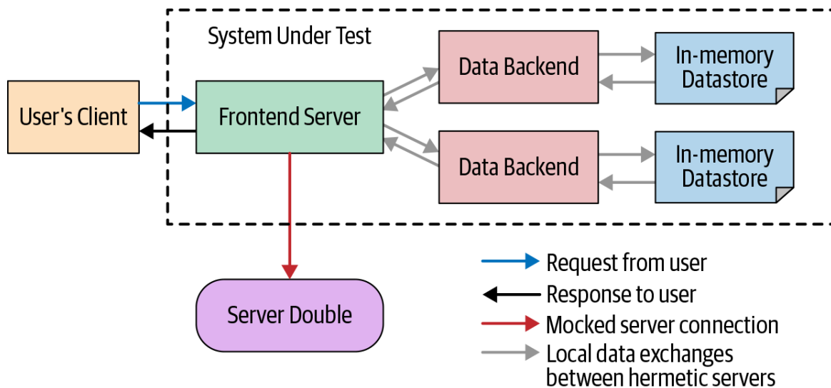
Figure 14-6. A reduced-size SUT
