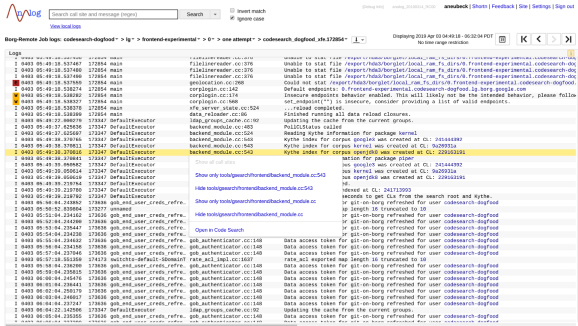
Figure 17-2. Code Search integration in a log viewer
