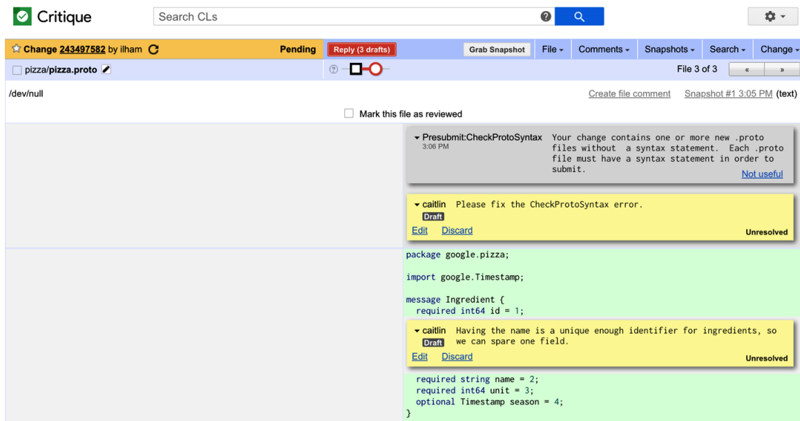
Figure 19-6. Commenting on the diff view
