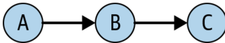
Figure 18-5. Transitive dependencies
