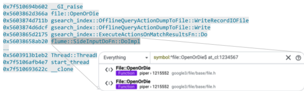
Figure 17-3. Code Search integration in stack frames
