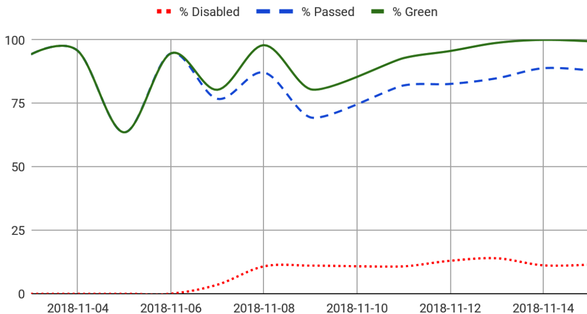
Figure 23-4. Achieving greenness through (responsible) test disablement
