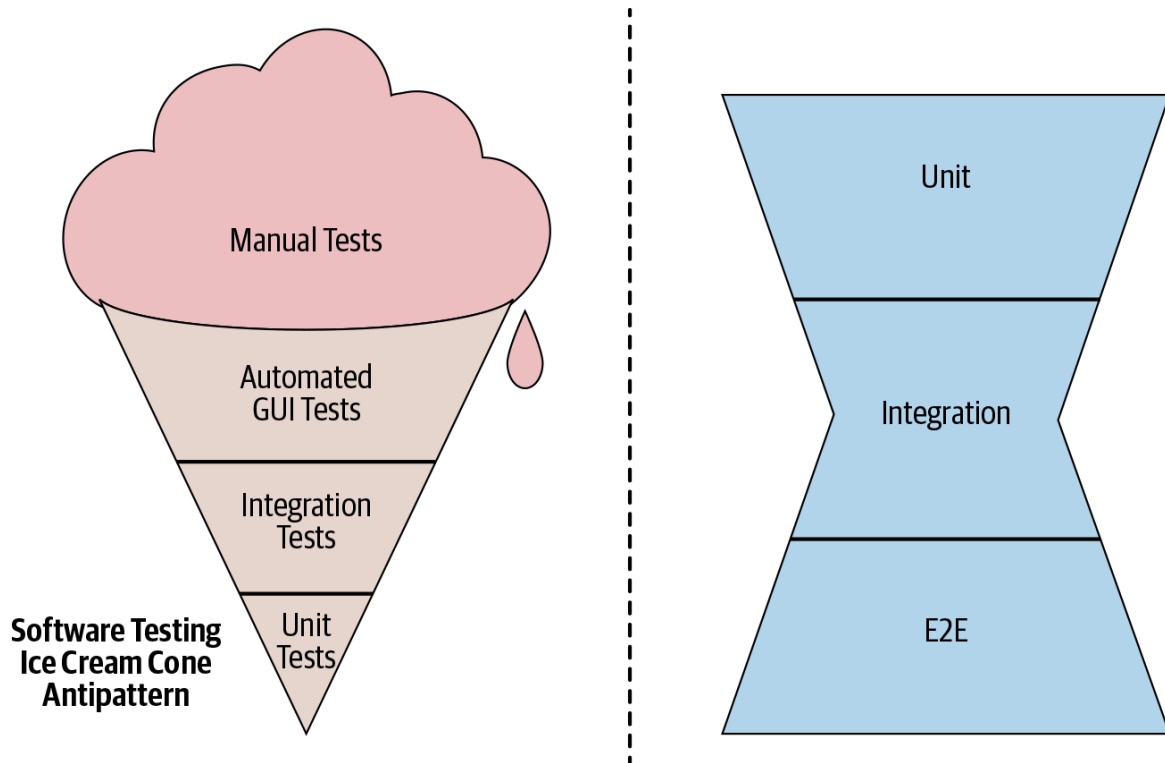
Figure 11-4. Test suite antipatterns
