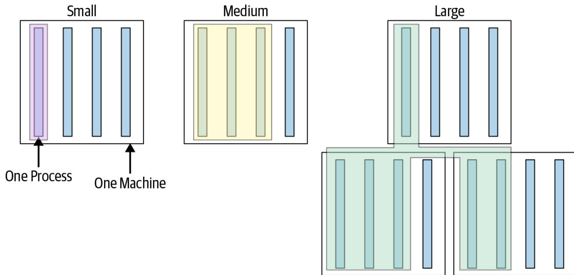
Figure 11-2. Test sizes
