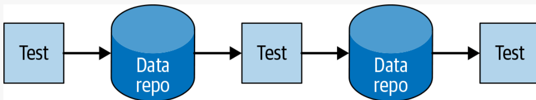
Figure 14-4. Chained tests
