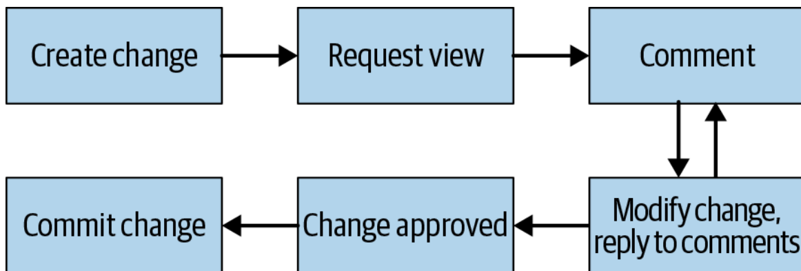
Figure 19-1. The code review flow
