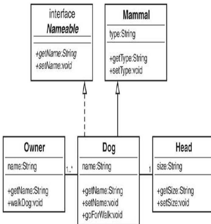
Figure 9.9 A UML diagram for the Dog example.
