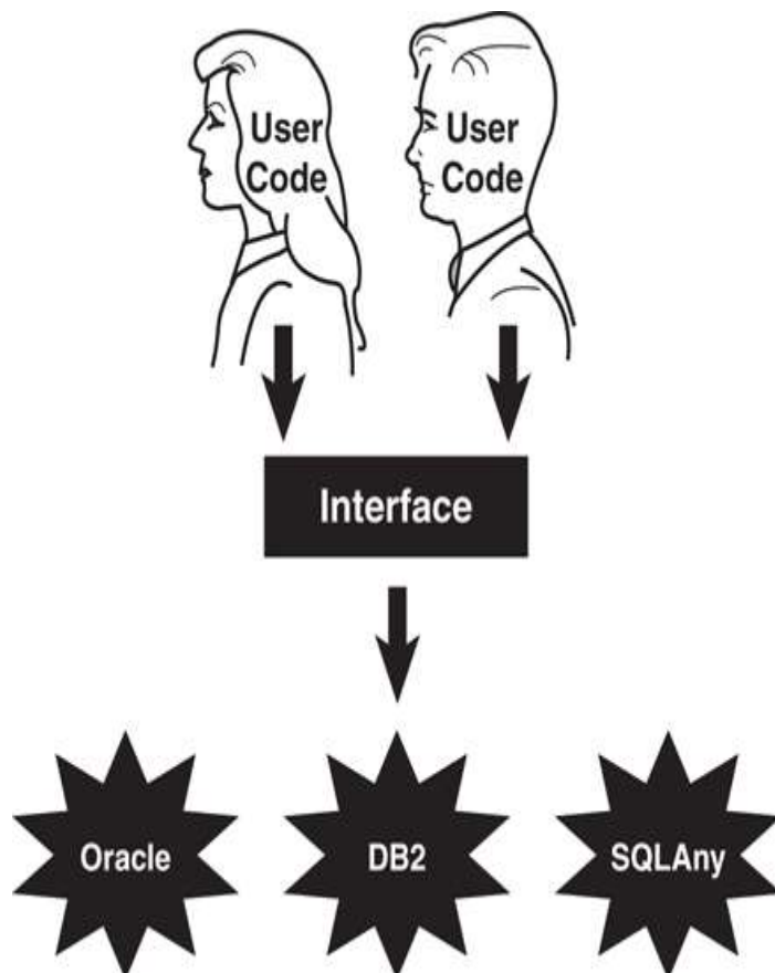
Figure 2.3 The interface.
