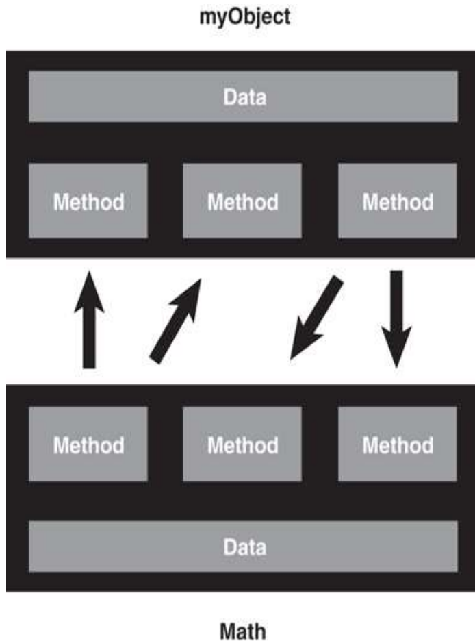
Figure 1.3 Object-to-object communication.
