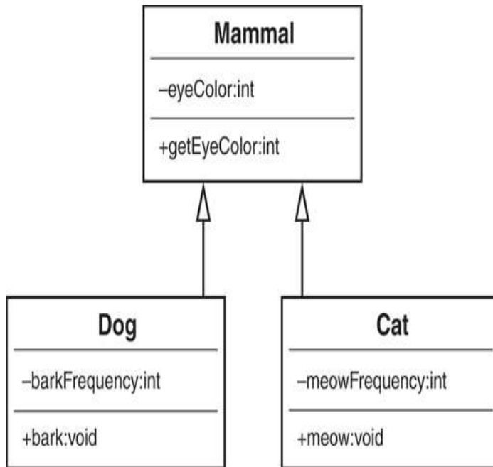
Figure 1.14 Mammal hierarchy.
