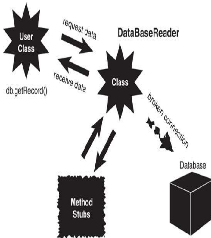
Figure 5.6 Using stubs.
