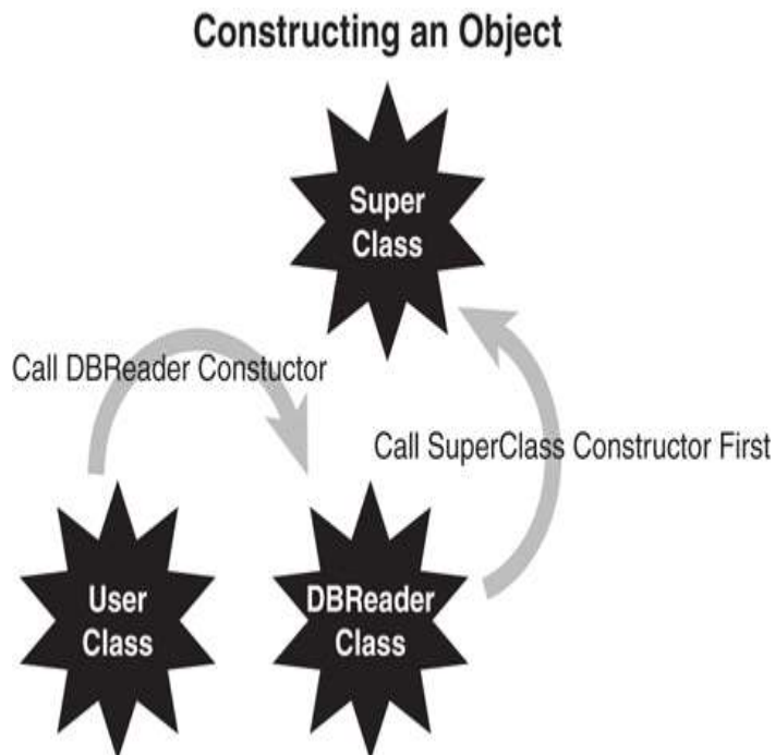
Figure 3.4 Constructing an object.
