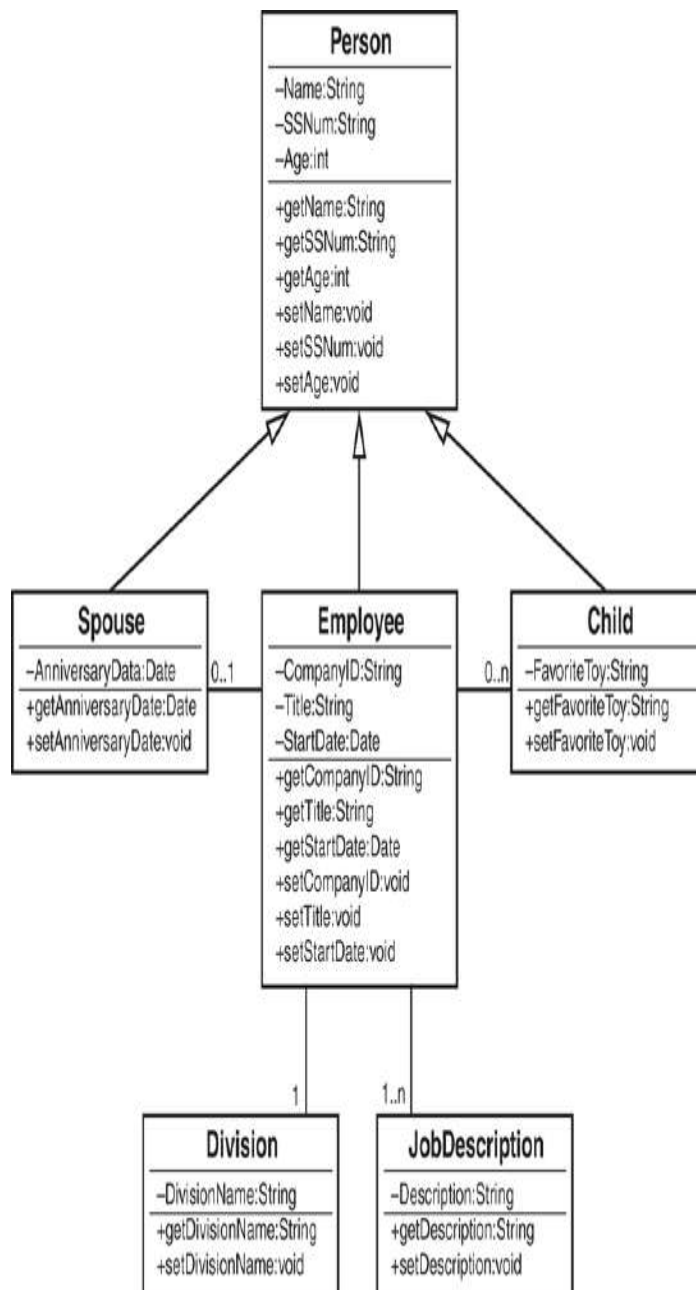
Figure 9.7 Cardinality in a UML diagram.
