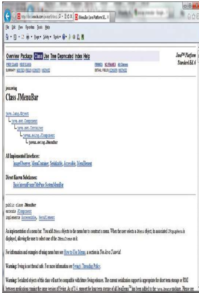
Figure 8.2 API documentation.
