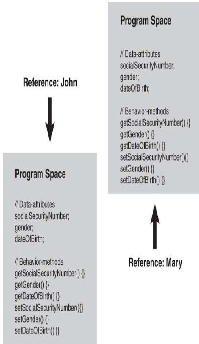
Figure 1.9 Program spaces.
