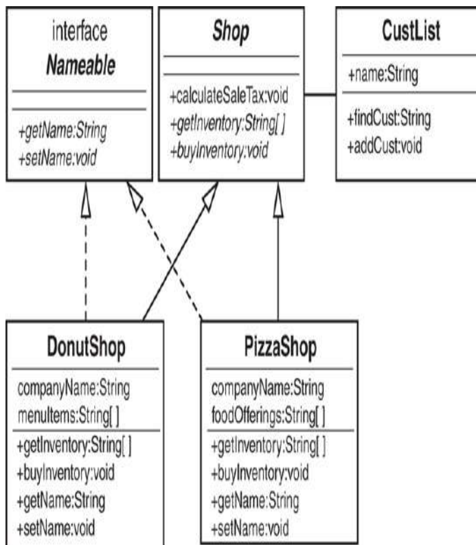
Figure 8.7 A UML diagram of the Shop model.
