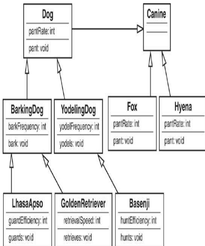
Figure 7.5 An expanded canine model.
