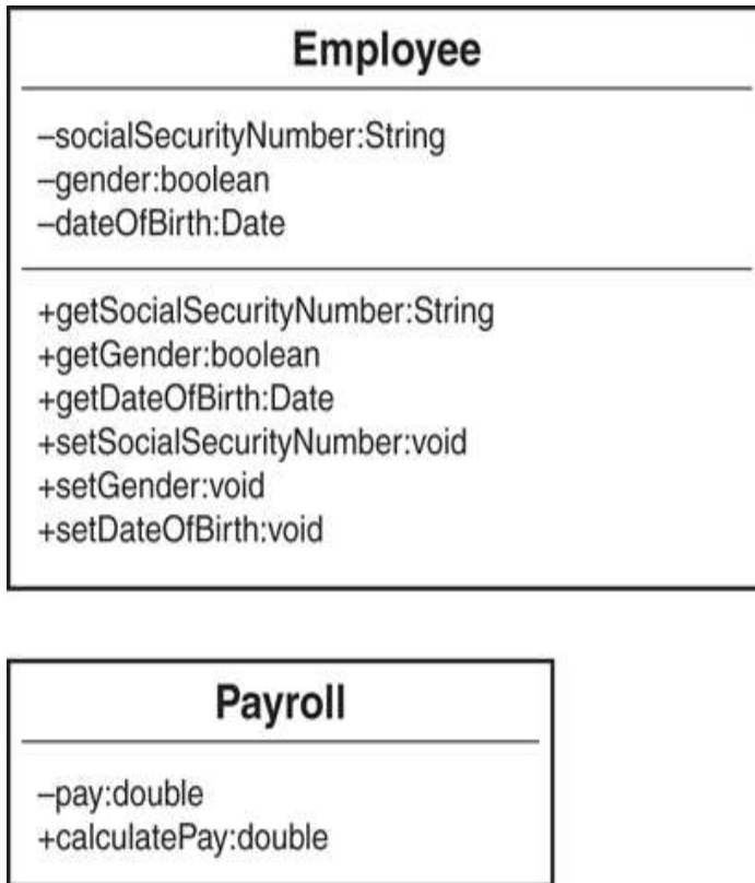
Figure 1.8 Employee and payroll class diagrams.
