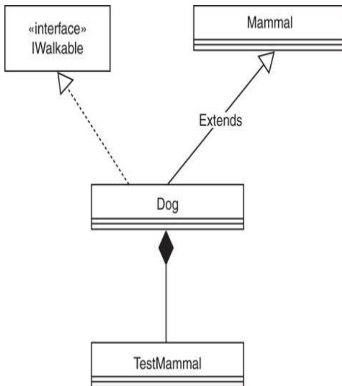
Figure 11.3 Using interfaces to create mammals.
