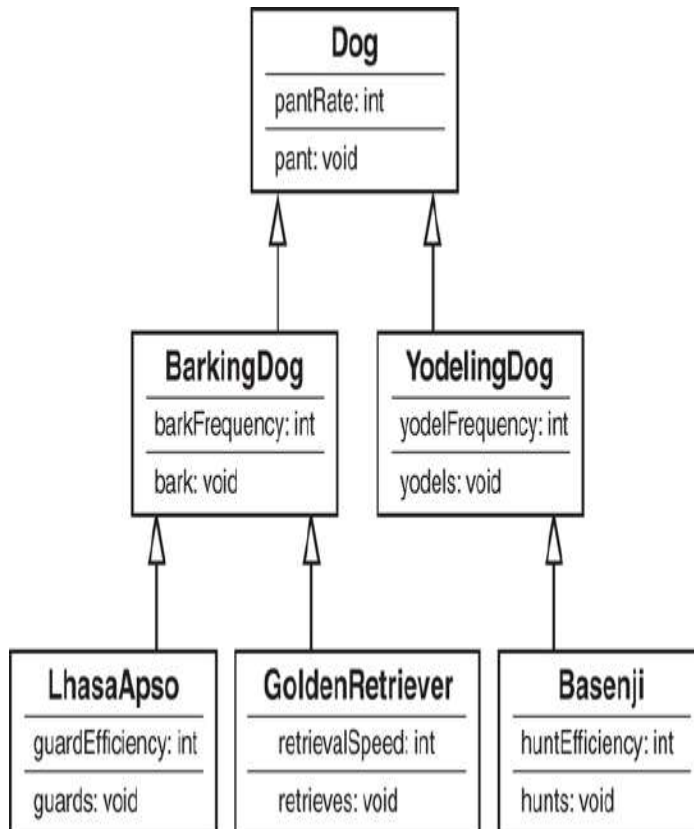
Figure 7.4 The Dog class hierarchy.
