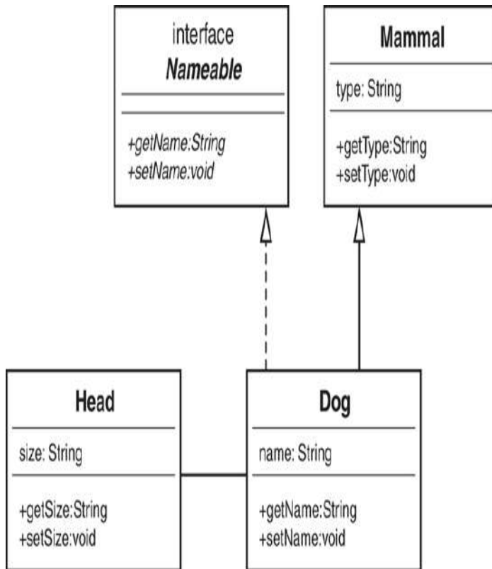
Figure 8.5 A UML diagram of the sample code.
