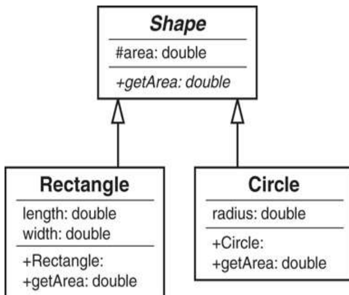
Figure 7.11 The Shape class hierarchy.
