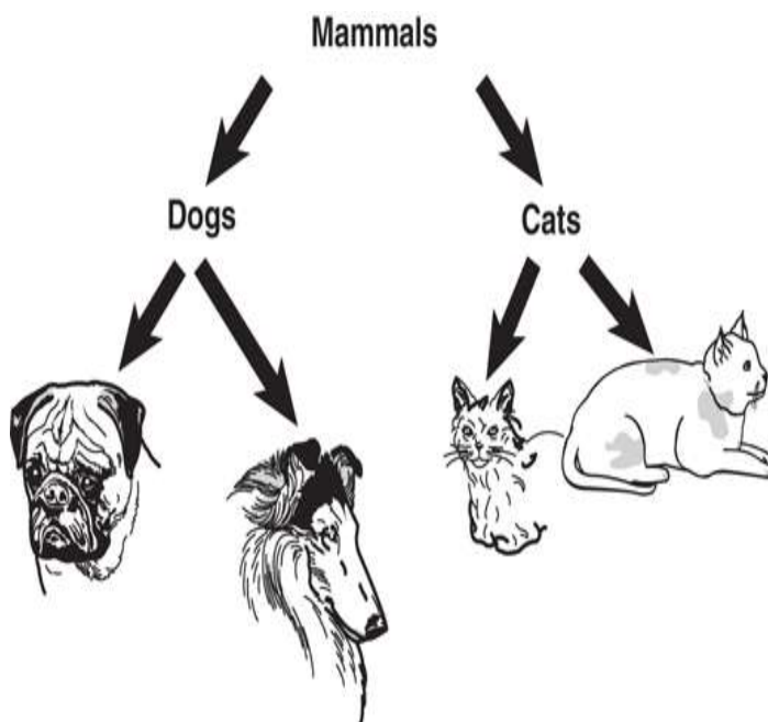
Figure 1.16 Mammal hierarchy.
