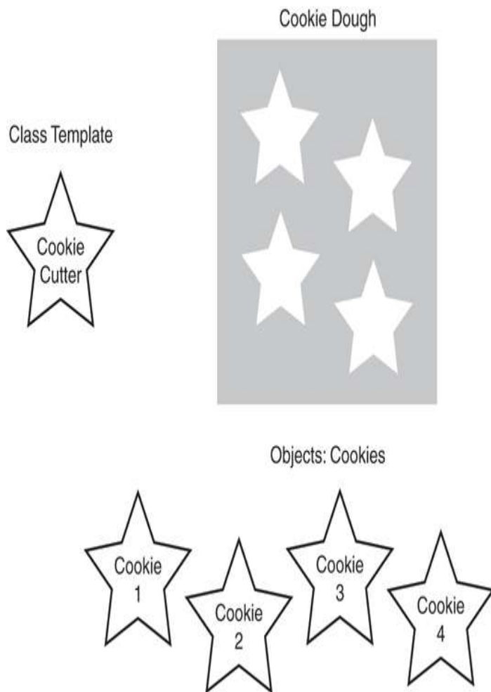
Figure 1.10 Class template.
