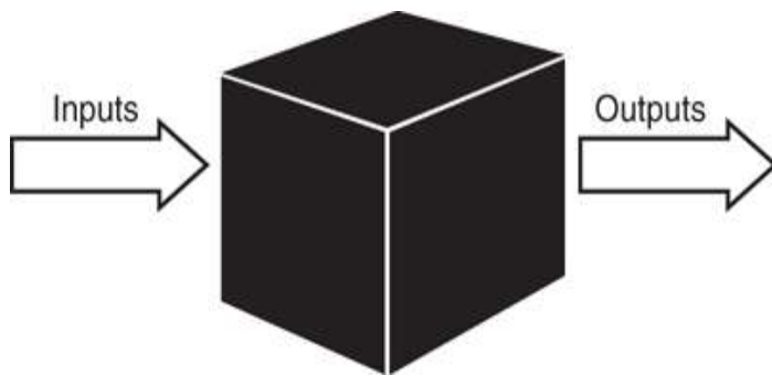
Figure 1.1 Black boxes.
