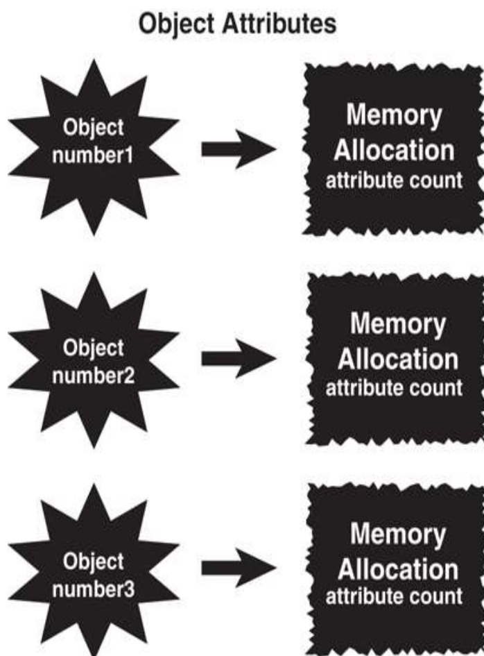
Figure 3.6 Object attributes.
