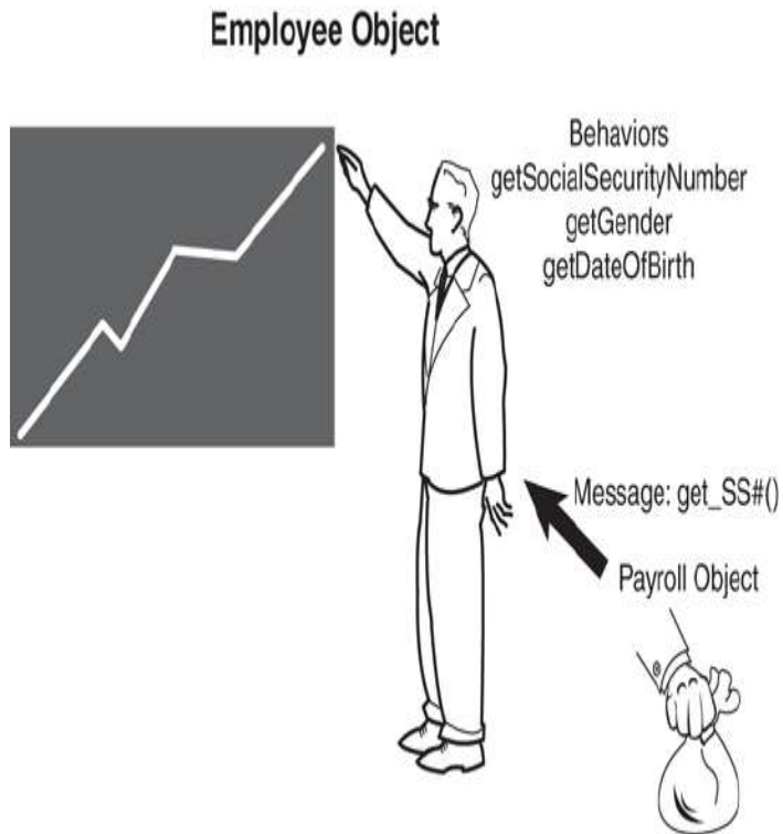
Figure 1.7 Employee behaviors.
