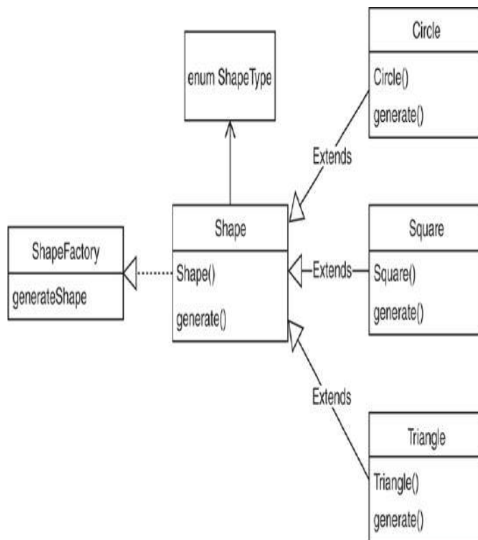
Figure 10.2 Creating a factory for the Shape class.
