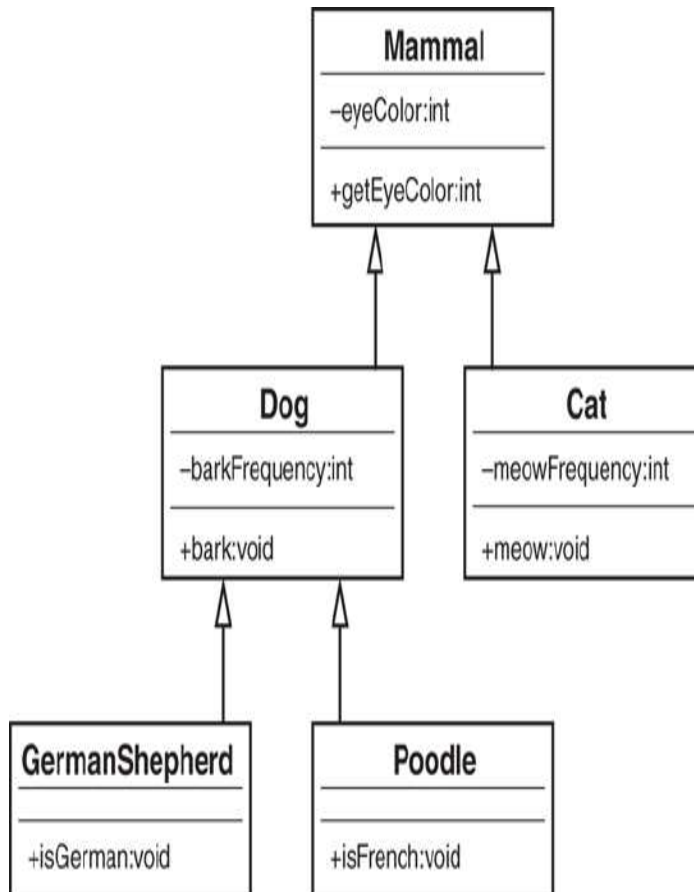
Figure 1.15 Mammal UML diagram.
