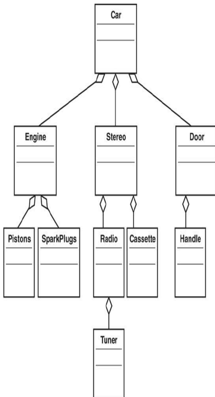
Figure 9.4 An aggregation hierarchy for a car.
