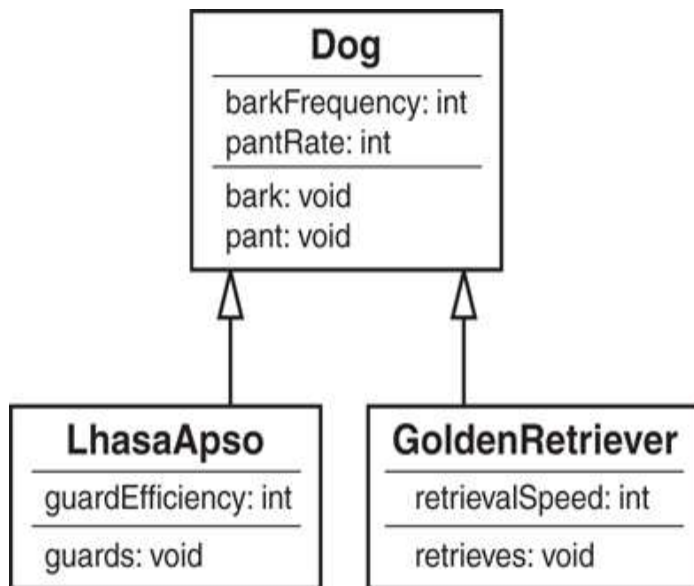
Figure 7.3 The LhasaApso class inherits from the Dog class.
