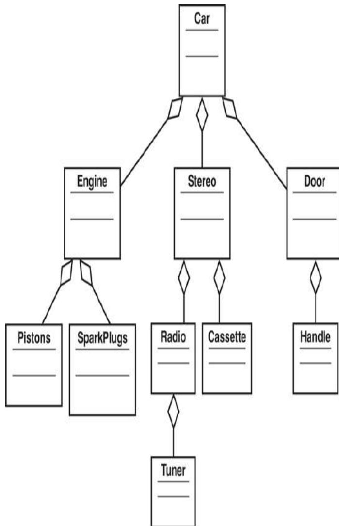
Figure 7.8 The Car class hierarchy.
