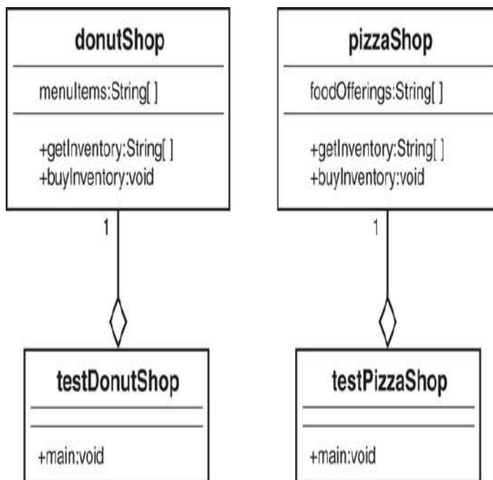
Figure 8.6 Applications on divergent paths.
