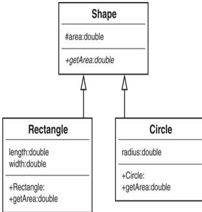
Figure 1.18 Shape UML diagram.
