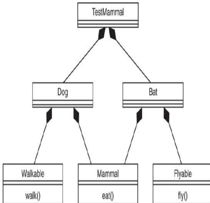
Figure 11.2 Using composition to create mammals.
